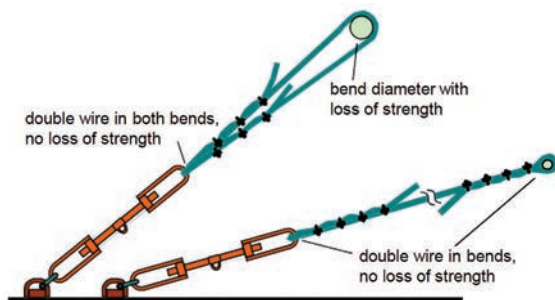
Figure 7.14 Recommended assemblies for wire rope lashing
