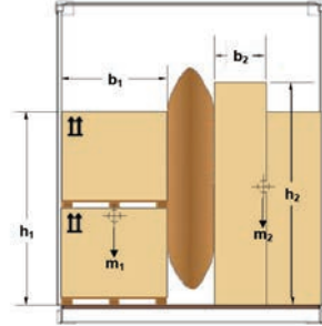
Figure 7.60 Unequal height packages
