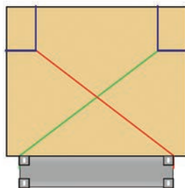
Figure 7.48 Transverse spring lashing
