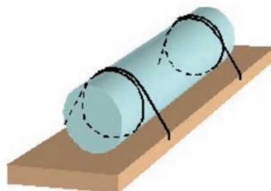
Figure 7.44 Silly-loop lashing
