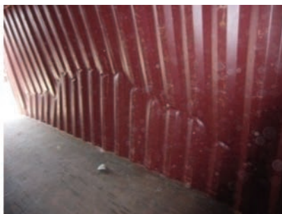
Figure 7.50 Damaged CTU side wall
