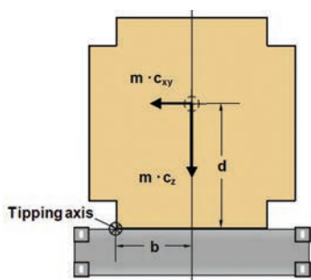
Figure 7.37 Tipping criterion
