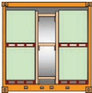
Figure 7.3 Centre gap with transverse bracing
