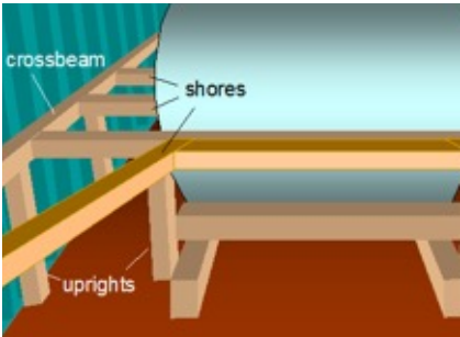
Figure 7.5 Shoring arrangement with uprights and crossbeam
