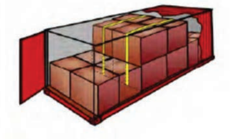
Figure 7.36 Round turn lashing
