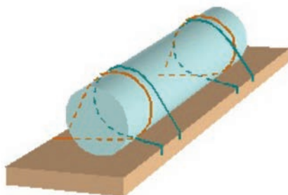
Figure 7.41 Vertical half-loop lashing
