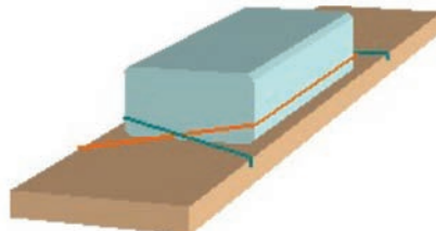
Figure 7.42 Horizontal half-loop lashing
